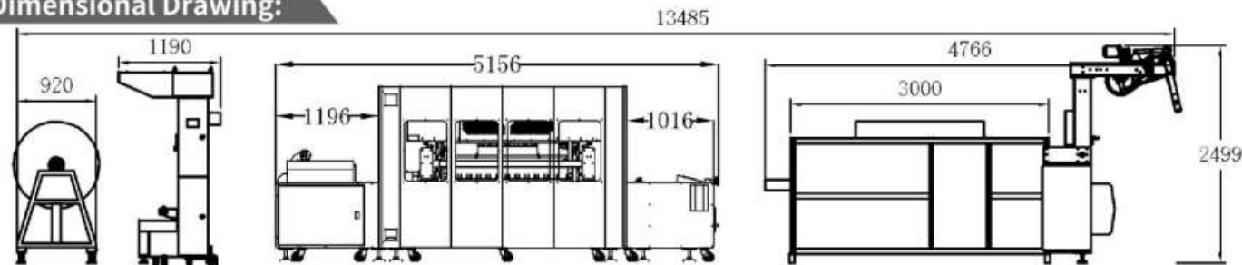
Dimensional Drawing:
